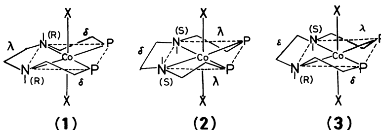
Fig. 2. Three possible diastereomers of \text{trans-}[\text{CoCl}_2(\text{SS-Me}_2\text{-pp-PNNP})]^+ .
